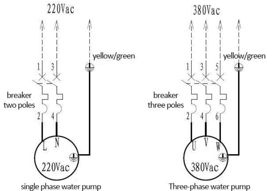
Figure 2-5: water pump connection diagram
