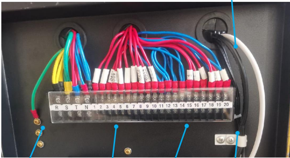
XT1 power input 400VAC 1-14: 230VAC 15-20: DC12V NTC temperature sensor (5K)
