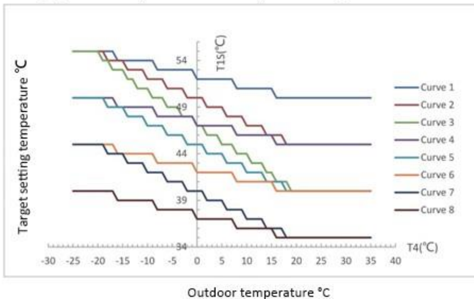
Heating high water temperature climate temperature compensation curve HH1-HH8
