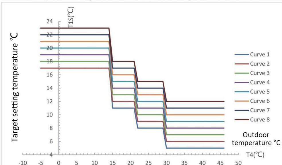
Cooling low water temperature climate temperature compensation curve CL1-CL8
